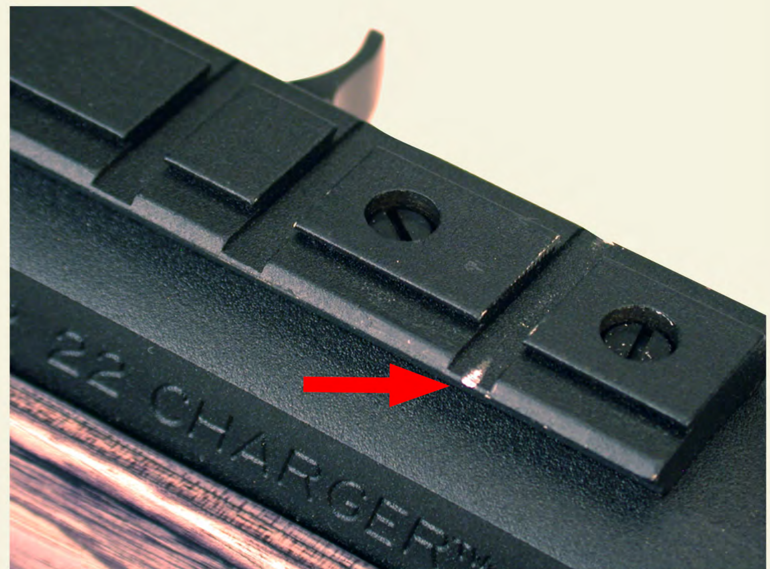
Above: The aluminum Weaver scope base was screwed down and coated with the same epoxy base matte coating. The base did not fit Picatinny mounts, and the coating rubbed off.
